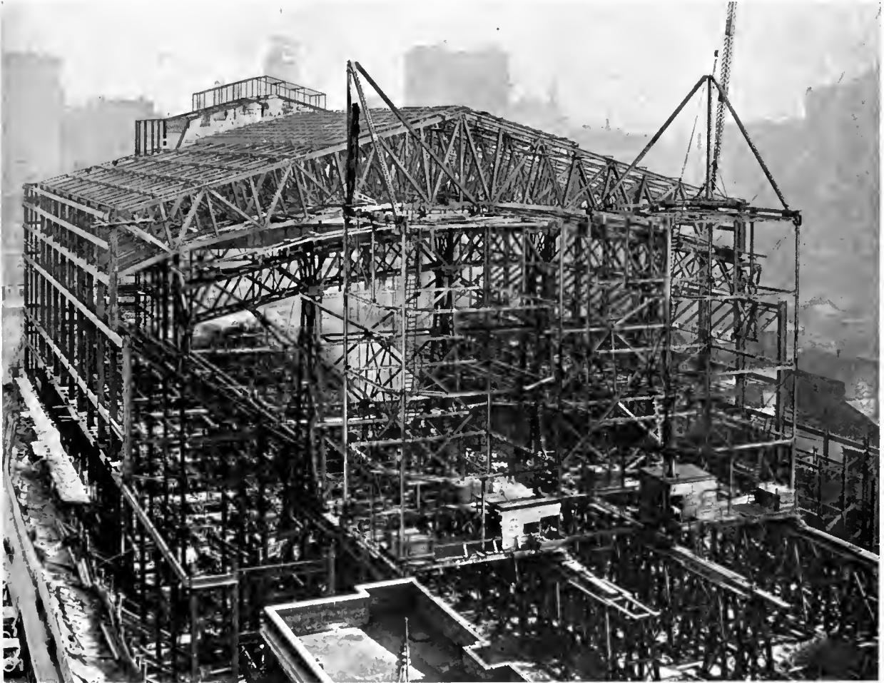
VIEW SHOWING PLANT USED IN THE ERECTION OF THE AUDITORIUM STEEL WORK
